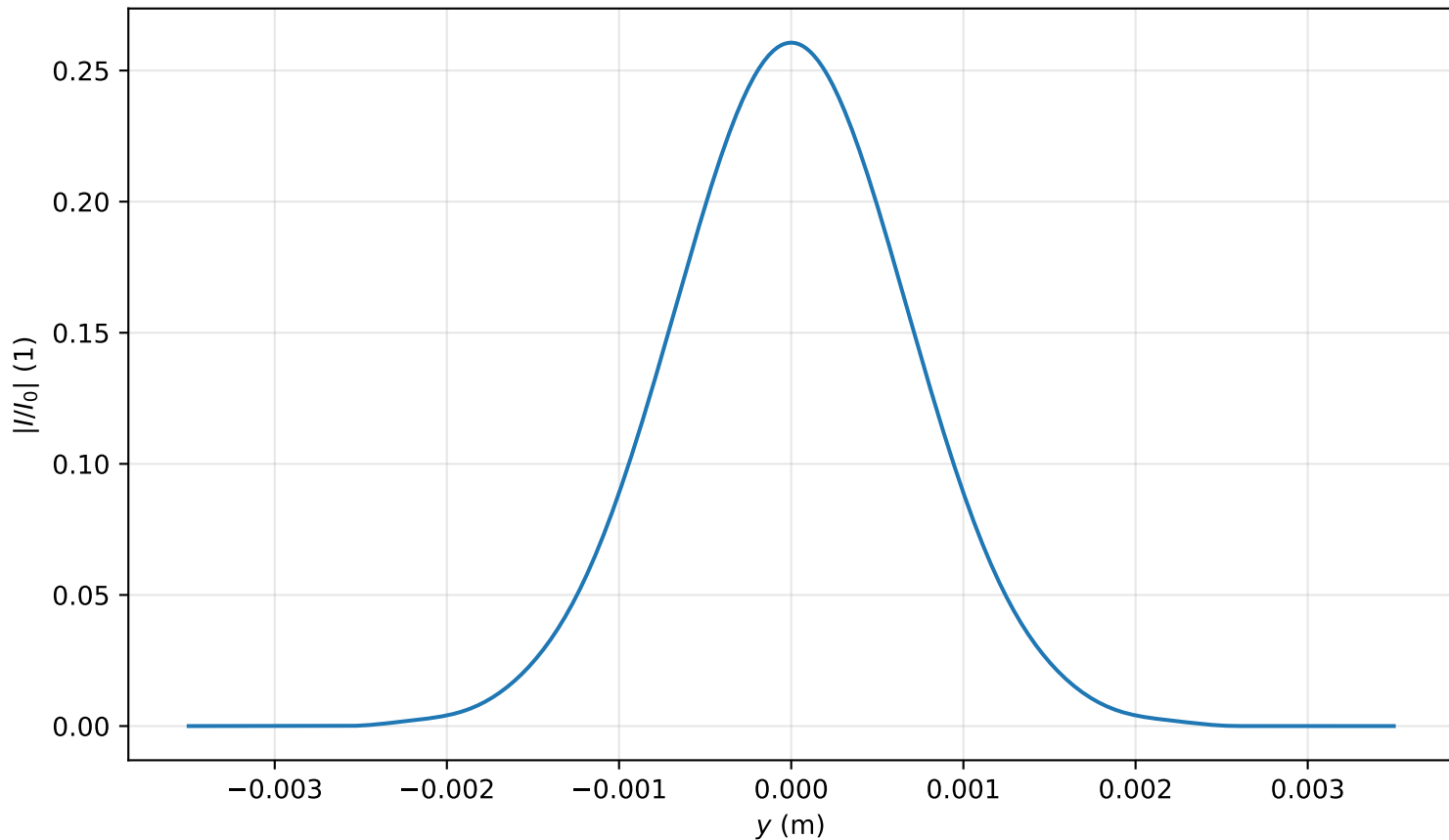
Intensity profile I(x=0, y, z=3.582)/I_0 , P_{in}=0.1P_{cr} , artificial time
